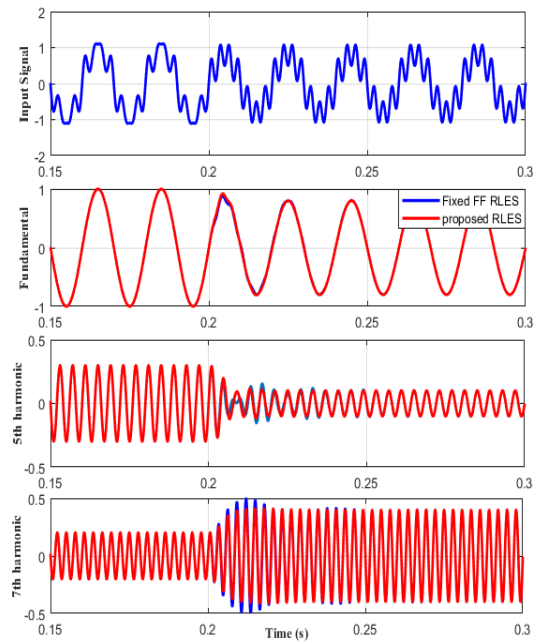
Fig. 5: Amplitude tracking changes of the fundamental, 5 th and 7 th harmonic components
