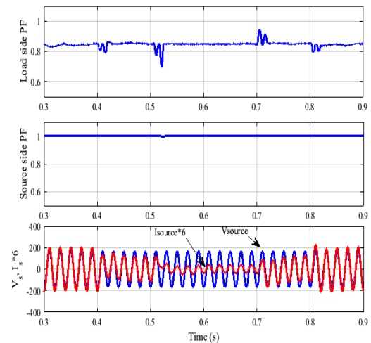
Fig. 14: DSTATCOM performance for power factor correction in case C
