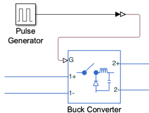
Fig. 13: Simulink buck converter model.
