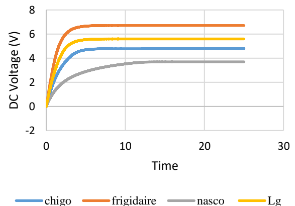
Fig. 19: Rectified output voltage at 17°C.
