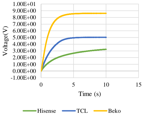
Fig. 16: Rectified voltage at 16°C.
