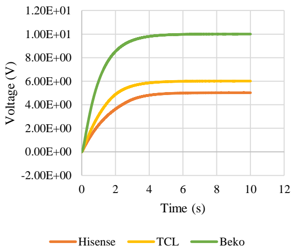
Fig. 18: Rectified voltage at 24°C.
