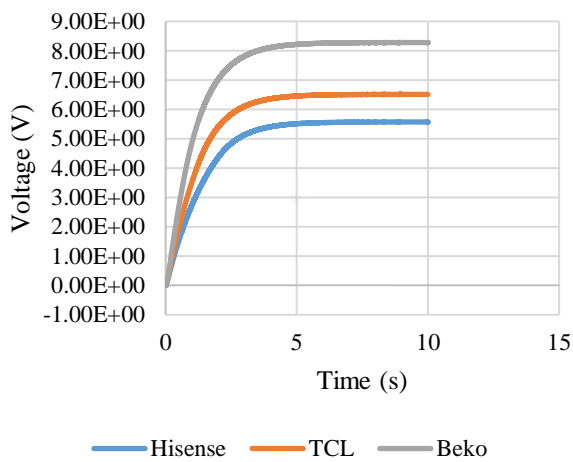
Fig. 17: Rectified voltage at 20°C.
